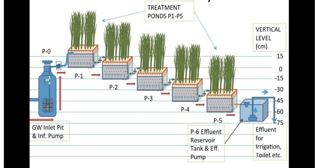
General scheme of the CW greywater (GW) treatment and reuse system
